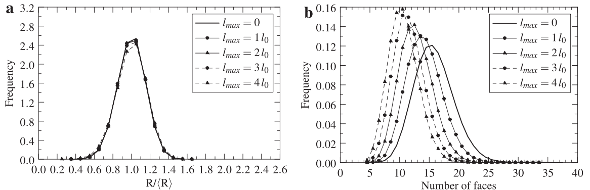
Fig. 7. Influence of the geometry regularization on the (a) distribution of grain size and (b) distribution of number of grain faces. R is the equivalent sphere radius. l_{max} is the length under which an edge is designated for deletion (with f_{max} = 20^\circ ). l_0 is the value of l_{max} considered in this article and is equal to 0.13 for grains of unit volume. For (b), the average values are 15.1, 13.7, 12.3, 11.1 and 10.2, respectively. Data collected on 10^5 grains.
