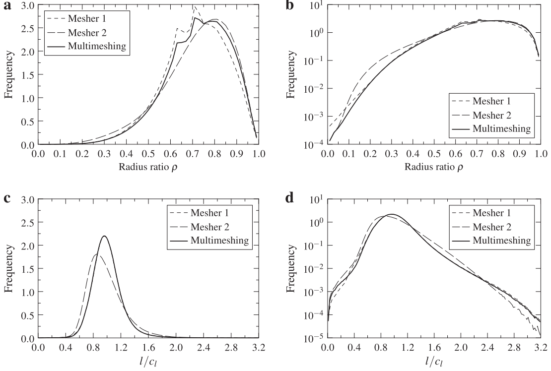
Fig. 11. Influence of the multimeshing strategy on mesh quality. Distributions of the (a–b) element qualities and (c–d) relative element sizes, in linear and logarithmic scales. Mesher 1 is the Netgen mesher + the Gmsh optimization; mesher 2 is the Netgen mesher + both the Netgen and Gmsh optimizations. Data collected on 10^5 grains.
