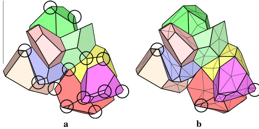
Fig. 4. Voronoi tessellation regularization: (a) original Voronoi tessellation and (b) equivalent regularized Voronoi tessellation. The small edges are surrounded and the face interpolations triangles are marked in gray. Case of a 9-grain polycrystal.
