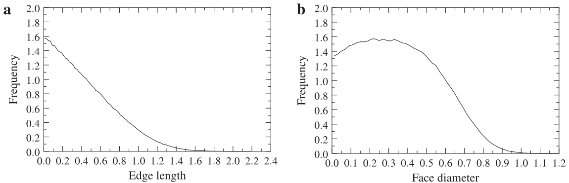
Fig. 3. Particular statistics of Voronoi tessellations. (a) Edge lengths, (b) face diameters. The data are given for grains of unit volume on average. The face diameter is based on the equivalent circle. Note the large number of small entities. Data collected on 10^5 grains.
