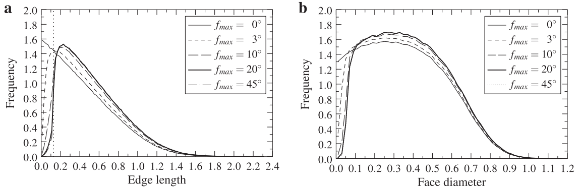
Fig. 5. Influence of the geometry regularization on the (a) edge length and (b) face diameter distributions, for increasing values of the maximum allowed flatness faults, f_{max} . On (a), the dotted line denotes the length under which the edges are considered to be “small” and so are designated for deletion. The data are given for grains of unit volume on average. The face diameter is based on the equivalent circle. Data collected on 10^5 grains.
