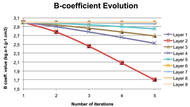
Figure 5. Evolution of the B coefficient of each layer through iterations.
