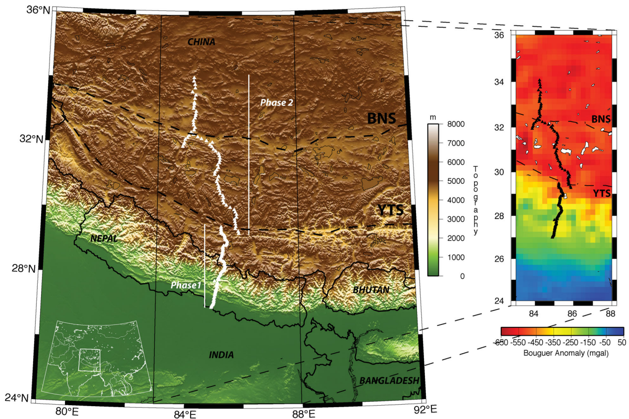
Figure 1. Topographic map of the Himalayan–Tibetan collision zone with the Hi-CLIMB temporary seismicological network (left-hand panel) and the Bouguer anomalies deduced from GOCE measurements (right-hand panel). On both maps, the black triangles represent the 152 stations of the Hi-CLIMB experiment’s main array, used for the joint inversion. The two dashed black lines mark the Bangong–Nujiang Suture (BNS) and the Yarlung–Tsangpo Suture (YTS).
