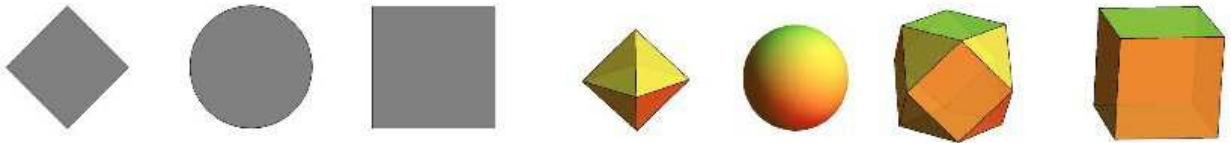
Figure 1: Structuring elements in 2D for the norms [\cdot]_1 = \ell^1 , \ell^2 , [\cdot]_0 = \ell^\infty and in 3D for the norms [\cdot]_2 = \ell^1 (octahedron), \ell^2 , [\cdot]_1 (cuboctahedron), [\cdot]_0 = \ell^\infty .
