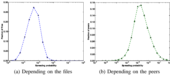
Fig. 7. Heterogeneous spreading parameter distributions
