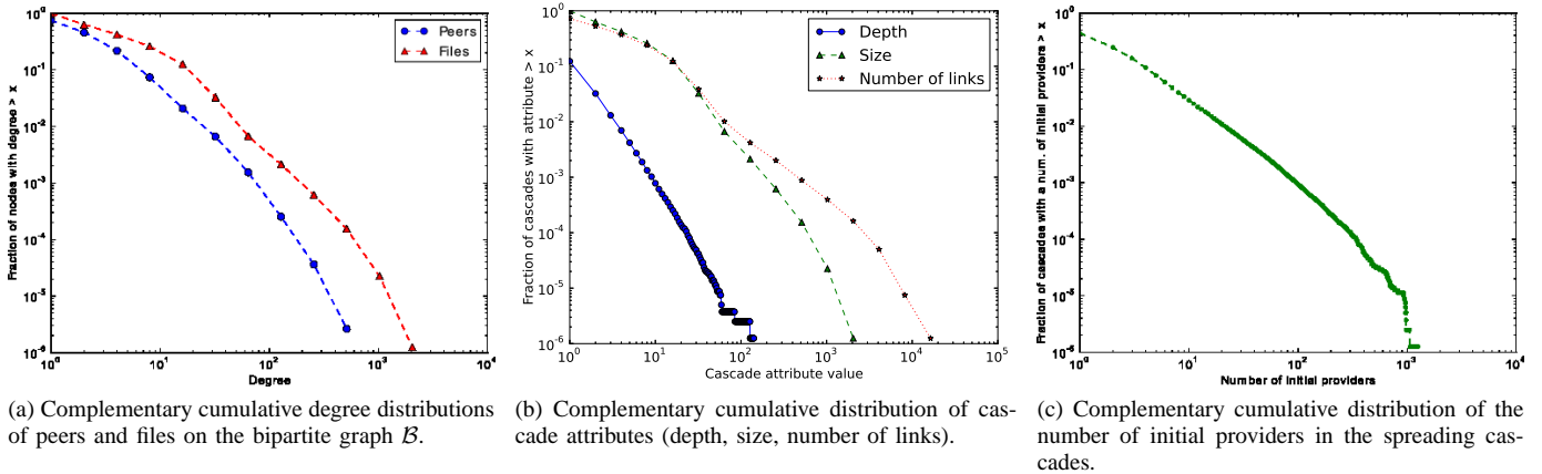
Fig. 2. Spreading statistics from the observed diffusion trace.
