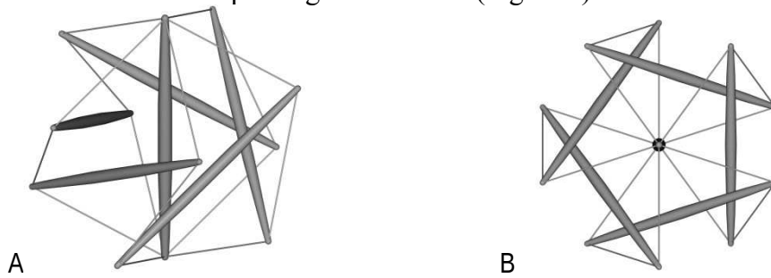
Figure 9: Spinning icosahedron: perspective and in plane views
