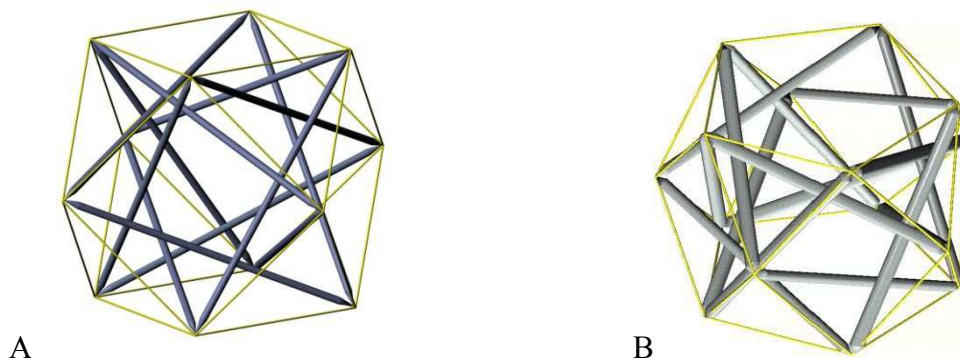
Figure 10: A-Cuboctahedron tensegrity system. B- Mono-circuit tensypolyhedron
