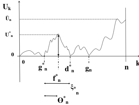
FIGURE 2. Notation U_n
