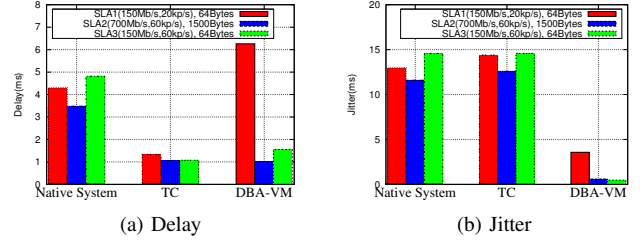
Fig. 6. Packets delay and jitter
