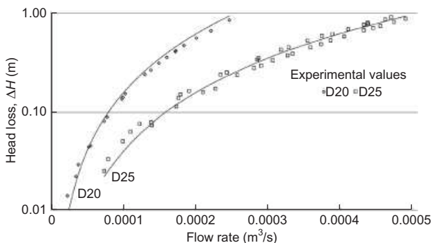
Figure 6. Discharge capacity of tubes. Solid lines are calculated head-loss curves. The slight scatter in the experimental values is due to measurement uncertainty
