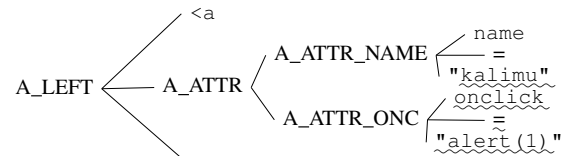
Fig. 4. Extract of the Parse Tree T_{G_o}(q(i_l)) of the SUT output q
