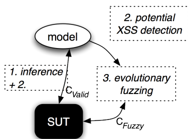
Fig. 1. Overview of our approach
