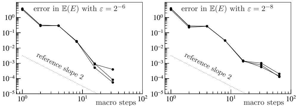
Figure 3: Multi-revolution methods for the FPU like problem (34) with Hamiltonian (35). Error in the Hamiltonian \mathbb{E}(E(P(T), Q(T))) (from top to bottom pictures, respectively) versus the number of macro steps (final time T = 2\pi ). The lines corresponds to the fully-discrete S-MRCM with n = 8, 16, 32 micro steps per macro step, respectively.
