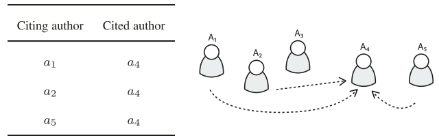
FIG. 3. Author citation network.
