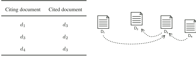
FIG. 1. Document citation network.
