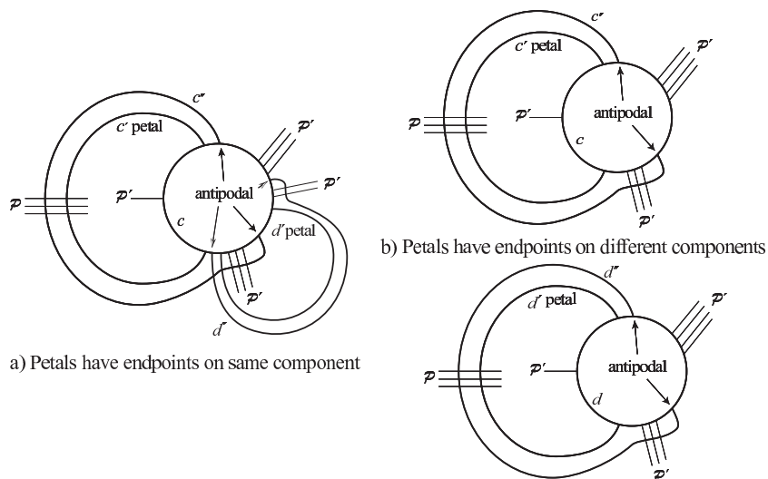
FIGURE 13. Construction of curves c'', d'' from petals of c', d' .
