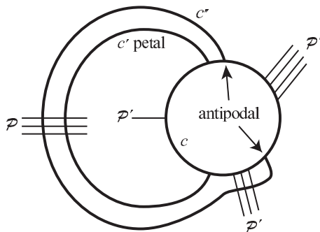
FIGURE 12. Construction of the curve c'' from a petal of c' .
