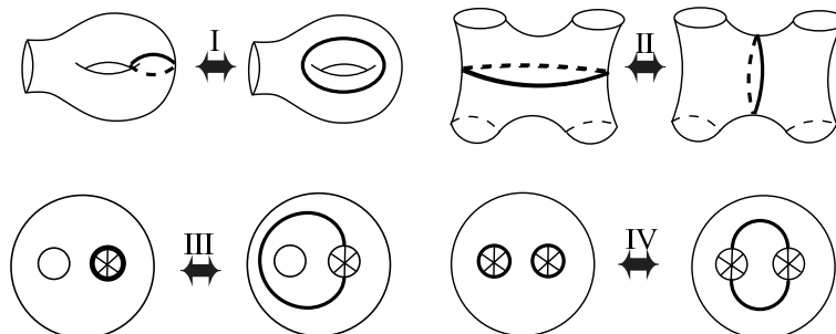
FIGURE 1. The four elementary moves. In each case, one or more of the depicted boundary components may bound a Möbius band both before and after the move. In Move III, a 1-sided curve is replaced by another 1-sided curve, and in Move IV, two 1-sided curves are replaced by a 2-sided curve or conversely.
