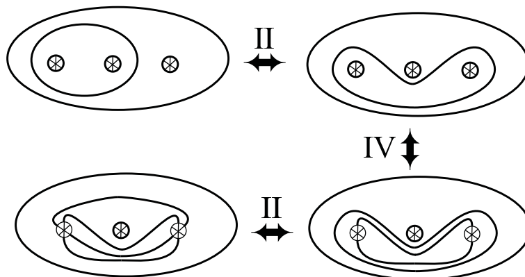
FIGURE 10. A sequence of moves in N_{3,1} preserving orientability and replacing three 1-sided pants curves and one 2-sided one by one 1-sided curve and two 2-sided curves.
