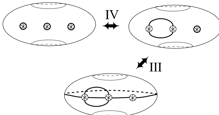
FIGURE 11. A sequence of moves in N_{3,0} preserving orientability and replacing three 1-sided pants curves by one 1-sided curve and one 2-sided curve.
