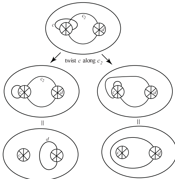
FIGURE 8. The effect on c of the right and left Dehn twists along c_2 in K_1 . One twist produces d whereas the other arises from move IV replacing d by the illustrated curve.
