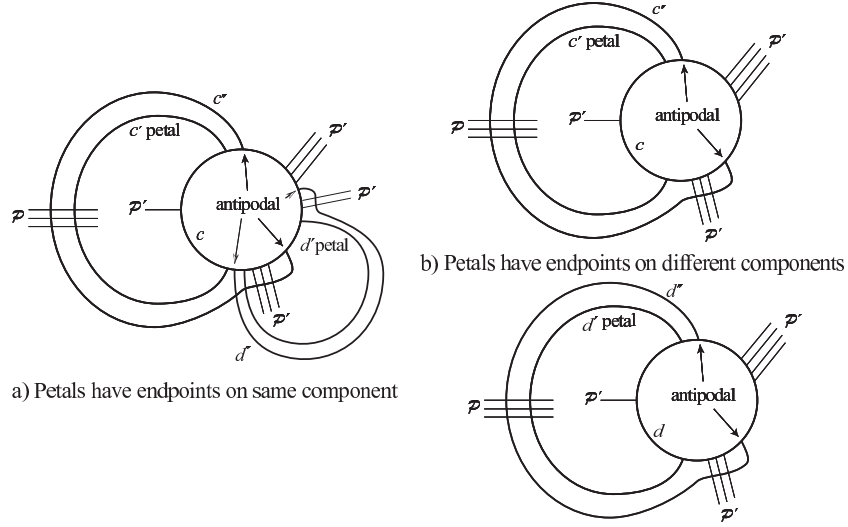
FIGURE 13. Construction of curves c'', d'' from petals of c', d' .
