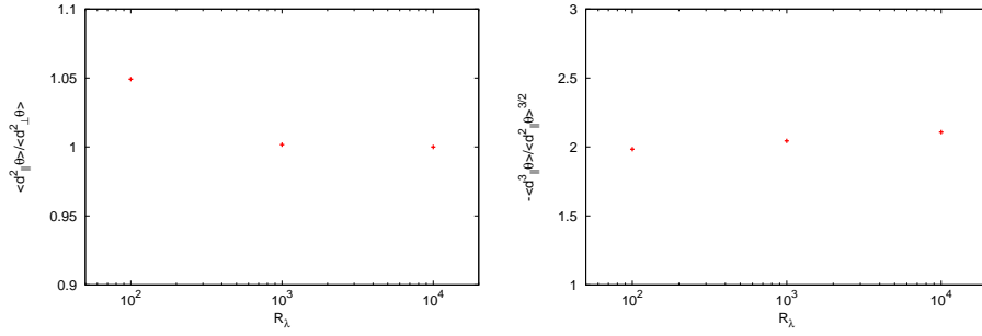
Figure 8: Left: Reynolds number dependence of the ratio of the mean-square parallel scalar gradients to the mean-square perpendicular gradients. Right: Reynolds number dependence of the parallel scalar gradient skewness.
