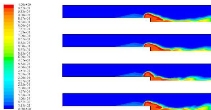
Figure 5: Mass fraction of Helium for 6666 Hz 25 % amplitude case at 1500, 1600, 1700 and 1800 iterations.
