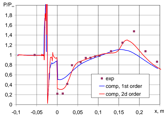
Figure 4: Experimental and computed pressure distributions along the central line on the bottom wall.
