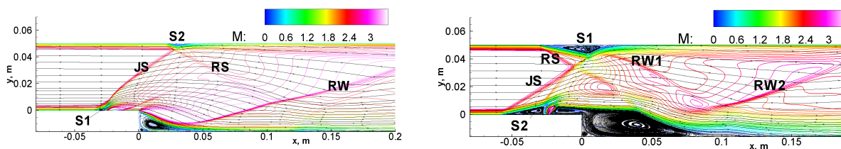
Figure 2: Mach contours and streamlines at different helium injection angles: left: \alpha=30^\circ and right \alpha=60^\circ
