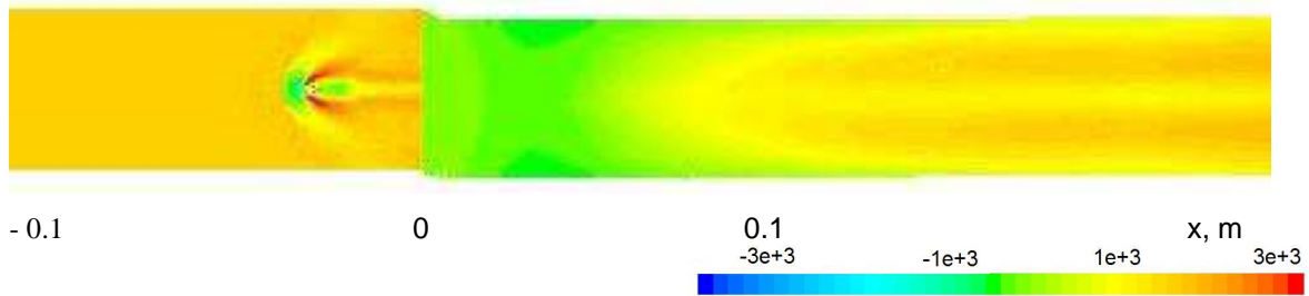
Figure 3: Shear stresses at the bottom wall of the model.
