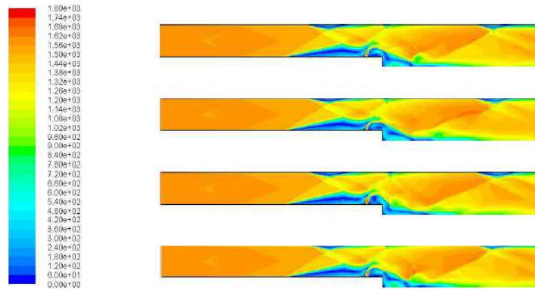
Figure 6: Velocity field for 6666 Hz 25 % amplitude case at 1500, 1600, 1700 and 1800 iterations, 0 - 1800 m/s.
