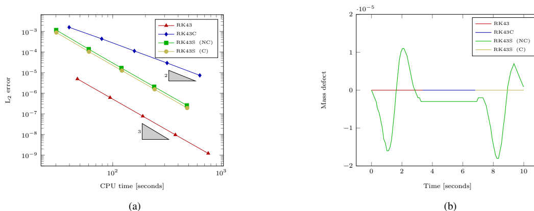
Figure 2: Convergence orders (a) and relative conservation defects (b).
