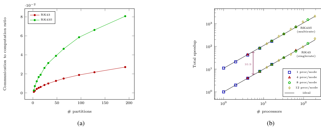
Figure 4: Estimation of the communication to computation ratio (a) and strong scaling (b) for RK43 and RK43S.
