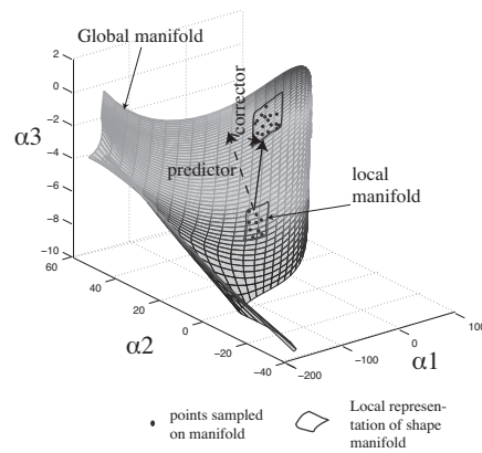
Figure 1: Shape manifold and local diffuse approximation
