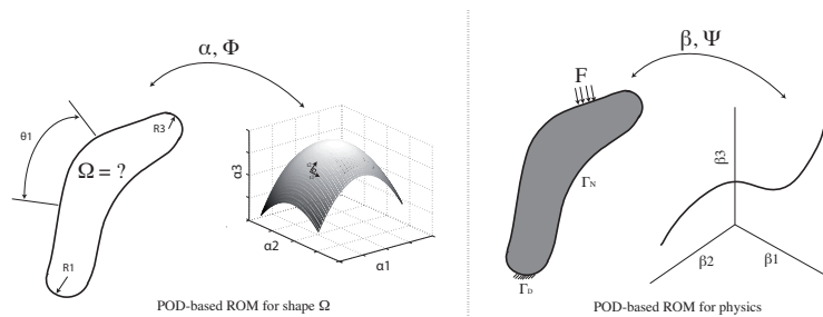
Figure 2: Basic idea of interactive design/optimization
