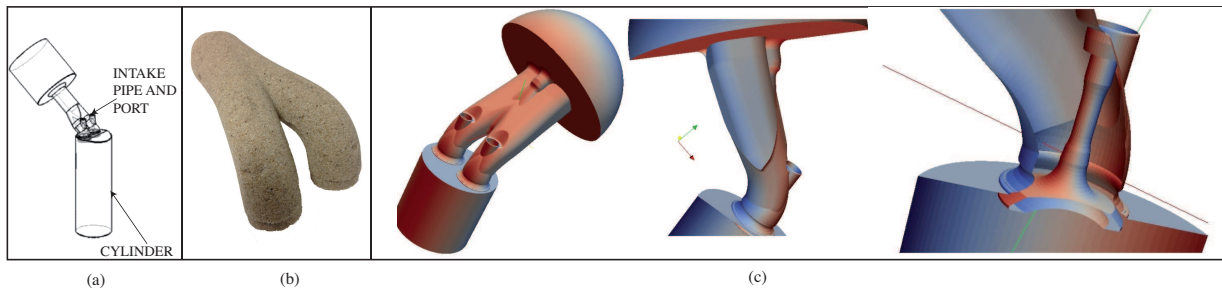
Figure 3: (a) Full system (b) Sand model of intake pipe (c) External & internal details of engine intake
