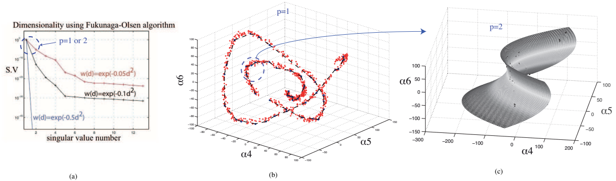
Figure 4: (a) Dimensionality p calculation, (b) Constrained shape interpolation using p = 1 , (c) \alpha -manifold approximation using p = 2 (normalized)
