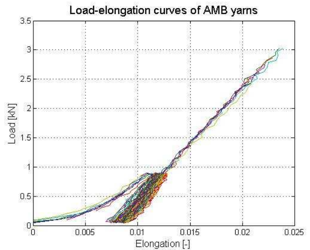
Figure 6. Yarn tensile test plots (5 samples)
