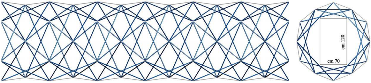
Fig. 24 The hollow rope (elevation and section)
