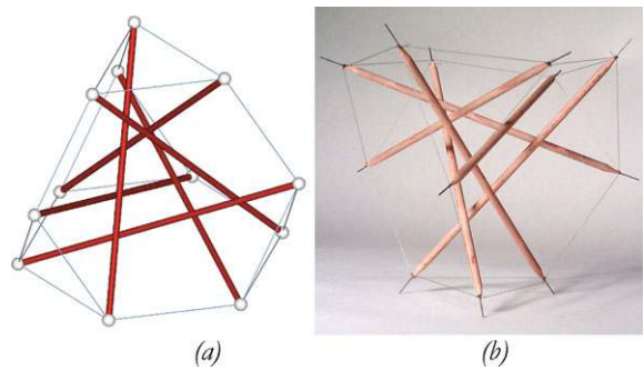
Fig. 4 Truncated tetrahedron with six struts inside (a—initial geometry and b—physical model)
