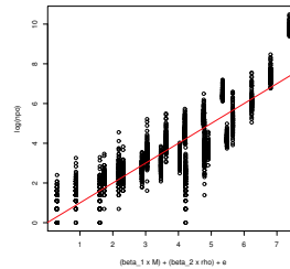
Fig. 2. Scatter plot of the linear regression model \log(\mathbf{npo}) = \beta_1 M + \beta_2 \rho + e , with \beta_1 = 1.30567 , \beta_2 = -2.87688 , and e = 0.27735 . Residual standard error: 1.037 on 3297 degrees of freedom, multiple R-squared: 0.7629, adjusted R-squared: 0.7627, F-statistic: 5303 on 2 and 3297 DF, p -value: < 2.2e - 16 .
