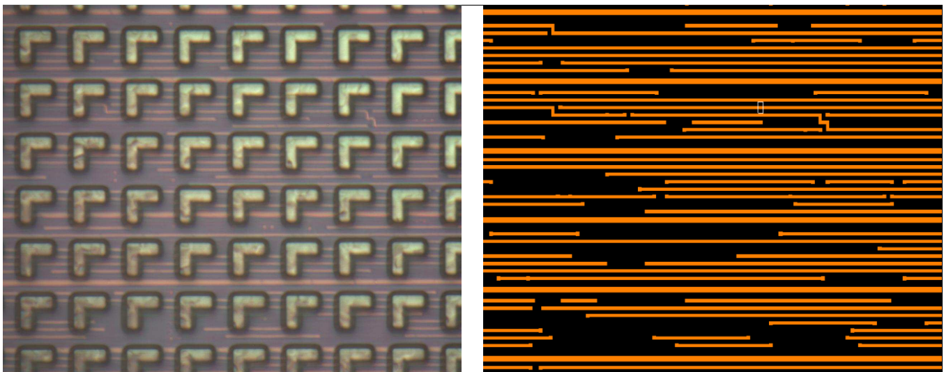
Figure 4. Picture (left hand side) and GDSII layout (right hand side – M6 in orange for Middle and Side of the module, M5 in yellow for Side of the module) of an AES-128 cryptographic accelerator (area size: 67 \mu\text{m} \times 60 \mu\text{m} )
