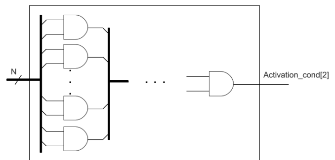
Figure 5. HTH with N - 1 AND gates (AND tree) inserted in AES circuit
