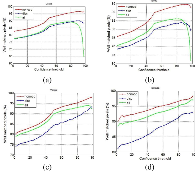
Fig. 6: Percentage of well-matched pixels vs. confidence measure threshold in non occluded regions (nonocc), all regions (all) and depth-discontinuity regions (disc) for (a) Cones, (b) Teddy, (c) Venus and (d) Tsukuba datasets.
