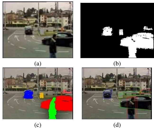
Fig. 12: Segmentation results using CICA (a) Original image (b) CICA segmentation result (c) Object localization obtained by stereo matching (d) Final 3D object localization.
