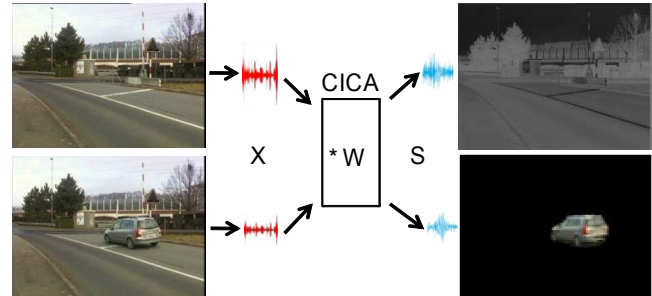
Fig. 1: Principle of the background subtraction using Independent Component Analysis. The input data is a combination of a reference signal, i.e. background image (top left image), and a given signal, i.e. an image from the sequence (bottom left image). ICA algorithm allows separating the input data into two independent signals: The one corresponds to the background model (top right image), the other corresponds to the estimated foreground without any details of the background (bottom right image).
