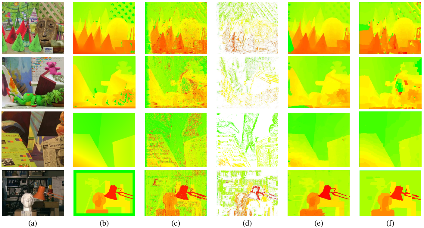
Fig. 8: Dense disparity map obtained with our algorithm compared to the max-product algorithm [14] (a) Standard test sets. Top to bottom: Cones, Teddy, Venus and Tsukuba (b) Ground truth for visual comparison. (c) Dense disparity map obtained applying the WACD likelihood function (d) Well-matched pixels having a confidence measure greater than 60% (e) Dense disparity map obtained from our algorithm (f) Dense disparity map obtained using the max-product formulation of the BP.
