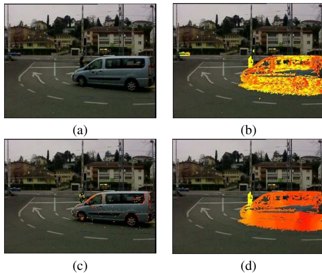
Fig. 11: Results obtained using HBP based on confidence measure (a) Left-hand image (b) Sparse disparity map obtained using WACD in the moving regions (c) Well-matched pixels estimated using the confidence measure with a threshold of 80% (d) Final disparity map.
