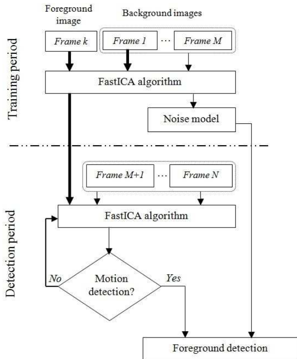
Fig. 2: Global scheme of the CICA model for the object detection module.
