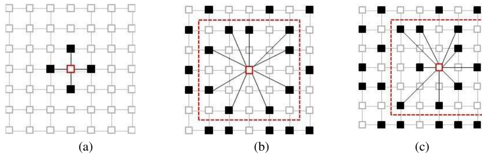
Fig. 7: (a) Standard messages passing principle of the belief propagation technique (b) iteration i of the proposed Hierarchical Belief Propagation (HBP) based on the k -nearest neighbors having high confidence measure (c) iteration i + 1 of the HBP. The black square points denote pixels having a confidence measure higher than a fixed confidence threshold. The confidence of a given pixel can be updated at the i^{th} iteration, and then can be used in the (i + 1)^{th} iteration.
