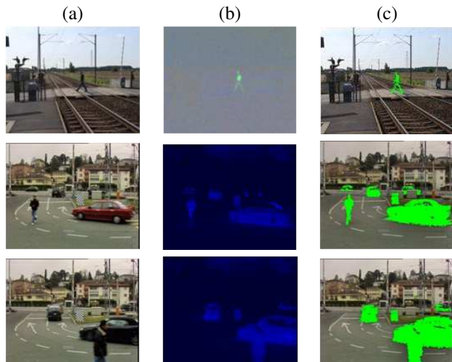
Fig. 5: Several objects at level crossings. (a) Original images containing pedestrians, cars and a stationary object (b) Estimated signal corresponding to foreground signal (c) Superimposition of the segmented moving objects into the original image.
