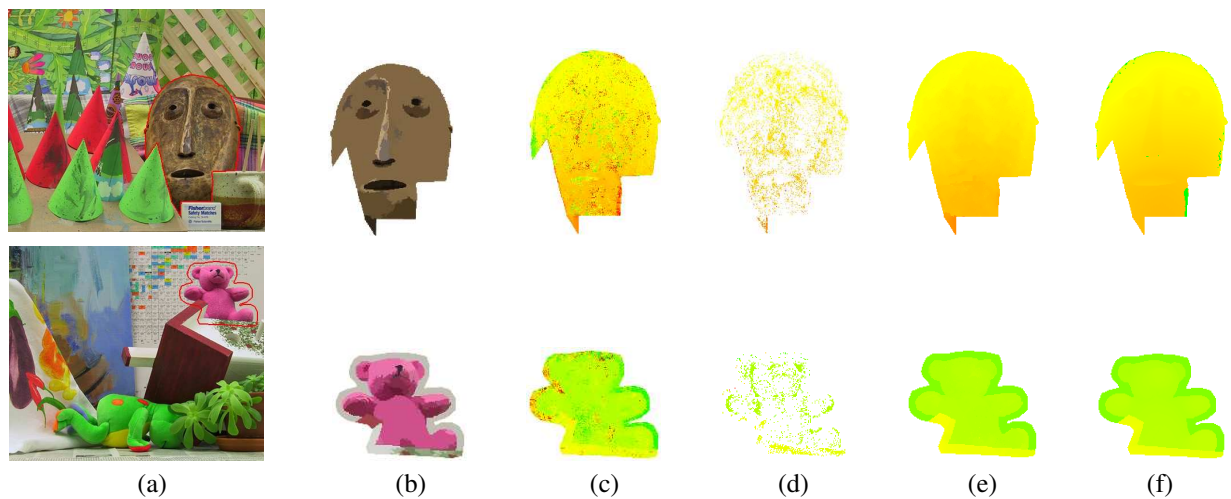
Fig. 9: Different steps of our algorithm in different types of regions. (a) Left image for Cones and Teddy (b) Segmented face and teddy bear extracted from the Cones and Teddy images, respectively, using Mean Shift (c) Dense disparity map obtained using WACD (d) Sparse disparity map corresponding to the well-matched pixels, with 60% confidence threshold (e) Dense disparity map after performing the HBP (f) Corresponding ground truth.
