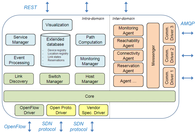
Fig. 2. DISCO Controller Architecture.
