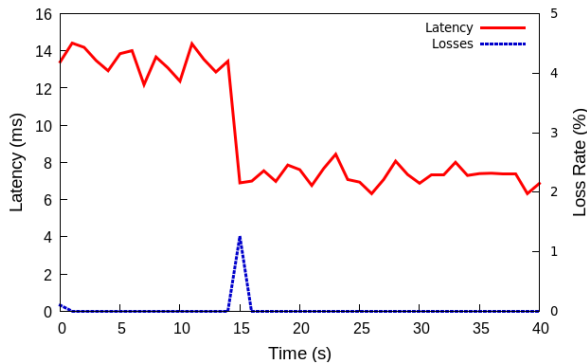
Fig. 9. Impact on flow latency and loss rate when the destination host 2 is moved from domain C to B.
