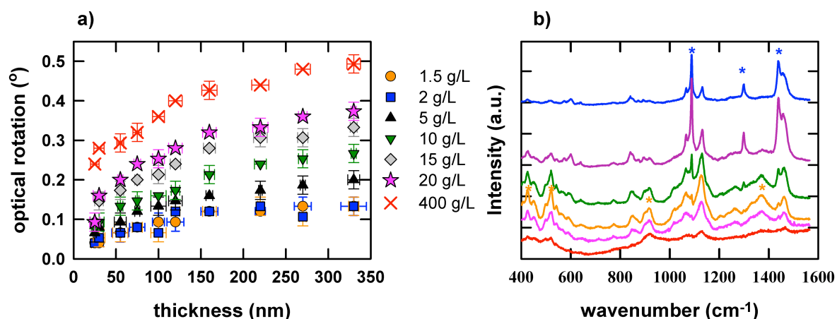
Fig. 1. Optical activity and Raman spectra. (a) Optical rotations of SDS+glucose films at a given 12 g/L SDS concentration for various glucose concentrations. (b) Raman spectra of SDS+glucose dried drops for different depths (from 0 to 5 \mu\text{m} with a 1 \mu\text{m} depth variation). The top spectrum is associated with the upper part of the sample. Blue and orange stars represent SDS and glucose contributions respectively.
