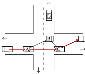
Fig. 7. An intersection scenario with only the furthest neighbor retransmitting (car C ), possibly missing to inform a crossing lane traffic (car D via car B ).
