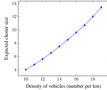
Fig. 5. Expected size of clusters, as a function of the vehicle density (with communication range of 200m).
