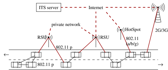
Fig. 2. Overview of the main set of interactions envisioned between vehicles and the infrastructure network.
