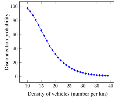
Fig. 4. Disconnection probability over 1km, for various vehicle densities (with communication range of 200m).
