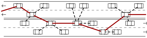
Fig. 8. CDS-based forwarding (general principle).
