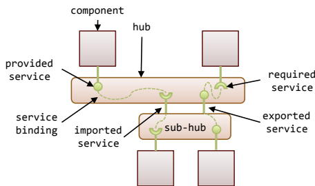
Figure 1. h-ubu application architecture
