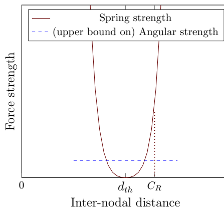
Figure 7: Priority between forces. Angular forces must prevail only when spring forces are nearly satisfied. An additional constraint is to ensure that the angular strength is always significantly lower than the spring strength at d_{th}/0.851 (minimal C_R ), so that angular forces cannot disconnect the network in case of conflicting configuration.
