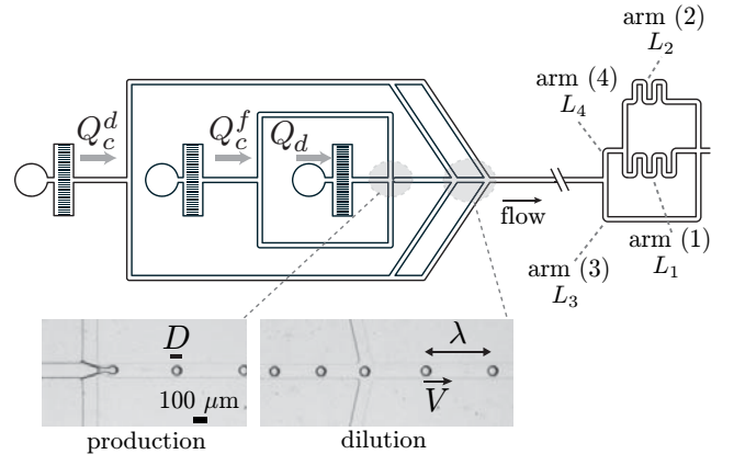
FIG. 15. Experiments: Schematic of the microfluidic device and photographs defining D , \lambda , and V .
