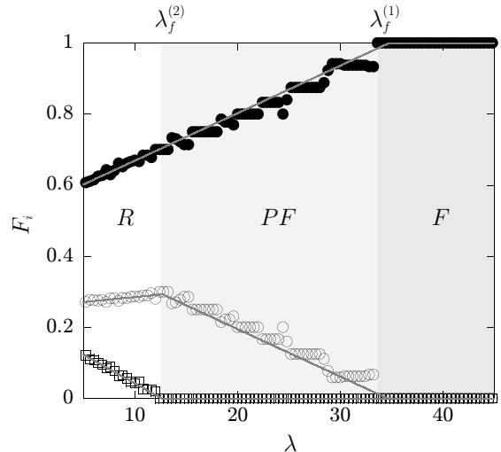
FIG. 7. Variations of F_1 ( \circ ), F_2 ( \square ), and F_3 ( \bullet ) with \lambda . The parameters expressed in arbitrary units are L_1=L_3=100 , L_2=125 , L_4=60 , and L_d=2.7 ( L_{eq} > L_3 ). The solid lines are predictions calculated using the continuous model (see section III B). R , PF , and F respectively denote the Repartition, Partial Filter, and the Filter regimes.
