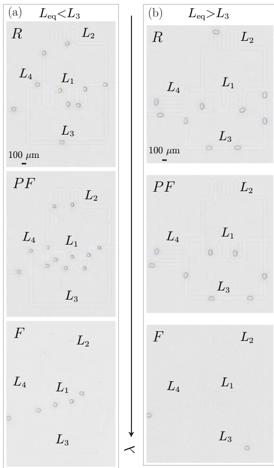
FIG. 16. Images of the three hydrodynamic regimes observed in imbedded loops when varying \lambda for (a, L_{eq} < L_3 ) L_1=L_3=4 mm, L_2=5 mm, L_4=1 mm and (b, L_{eq} > L_3 ) L_1=L_3=4 mm, L_2=5 mm, L_4=2.6 mm. The inlet and outlet of the loop are respectively located on the left and on the right of each image.
