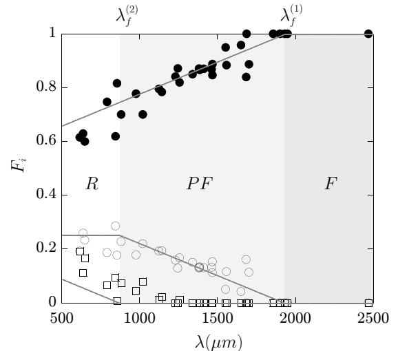
FIG. 17. Experimental variations of F_1 ( \circ ), F_2 ( \square ), and F_3 ( \bullet ) with \lambda in the configuration shown in Fig. 16(b). The solid lines are calculated using the continuous approach with L_d=165 \mu\text{m} in the Repartition and Partial Filter regime.
