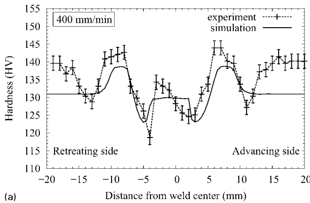
4 Experimental (dotted line) and simulated (continuous line) hardness profiles obtained on cross-section of AA 2024-T3 friction stir weld at 400 rev min -1 at rates of a 400 mm min -1 and b 100 mm min -1
