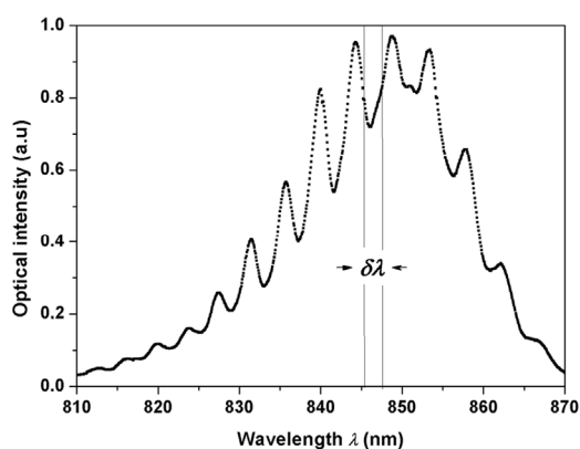
Figure 4. Optical spectrum of a 37 \mu\text{m} diameter spherical resonator with a Full width at half maximum, \delta\lambda = 2.25 nm.
