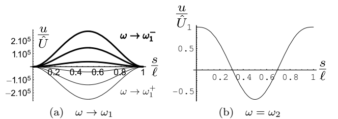
FIG. 10. Deflection u of a wall caused by the propagation of a wave in the x -direction with the X-mode. \hat{U} is the amplitude of the motion of the nodes, s is the coordinate along the axis of the wall, and \ell is the length of the wall.
