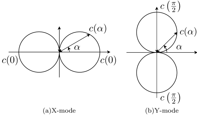
FIG. 8. Variations of the speed of the macroscopic waves according to the direction of propagation
