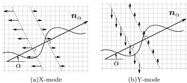
FIG. 6. Nodal displacements for the two modes of polarization
