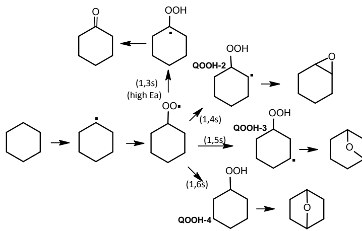
Fig. 4. Oxidation chemistry of the cyclohexyl radical (cy-C 6 H 11 ). Formation routes of C 6 H 10 O cyclic ethers and cyclohexanone.
