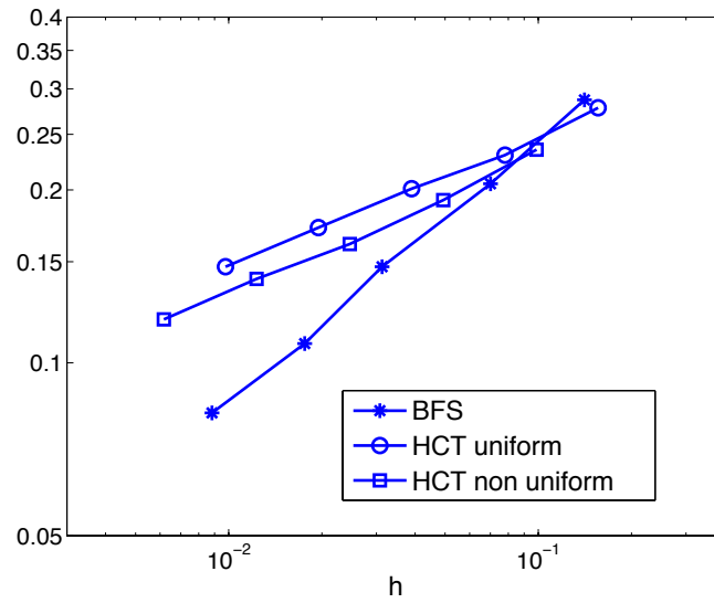
Figure 3: Example EX3 ; Evolution of \|v - v_h\|_{L^2(0,T)} w.r.t. h for BFS finite element ( \star ), HCT-uniform mesh ( \circ ) and HCT- non uniform mesh ( \square ); r = 1 .
