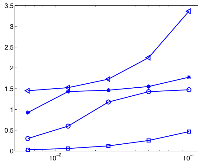
Figure 2: BFS finite element - Evolution of the inf-sup constant \delta_h with respect to h (see Table 2) for r = 10^{-4} (<), r = 10^{-3} (*), r = 10^{-2} (o) and r = 10^{-1} (square).
