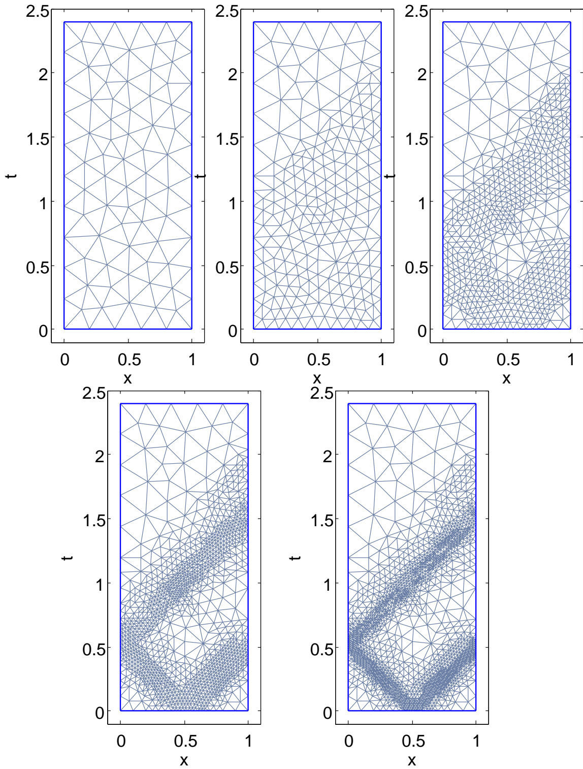
Figure 7: Example EX3 - Iterative refinement of the triangular mesh over Q_T with respect to the variable \lambda_h : 142, 412, 1 154, 2 556, 4 750 triangles; r = 2 \times 10^{-3} .
