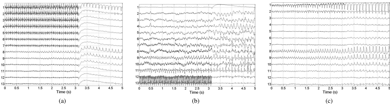
Fig. 15: Elimination of the stimulation and baseline artefacts from SEEG data with an epileptic activity during DBS (DBS ends at 3.1 s). (a) - real SEEG as registered with the epilepsy during DBS. (b) - sources after SSA-GEVD decomposition. (c) reconstructed signal eliminating the first and the last two components.
