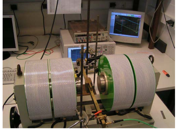
Fig. 8. Experimental test device.
