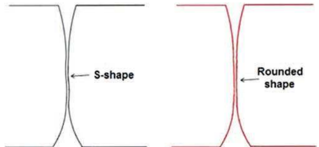
FIG. 5. Actual MLC leaf edge (left) and MLC leaf edge approximation as simulated with GATE. The small "S shape" at the center is not taken into account in the simulation because exact curvature and dimensions were not made available.
