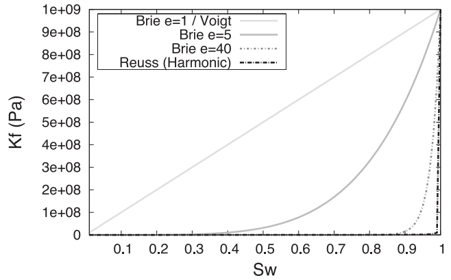
Figure 2. Effective bulk modulus K_f for a water–air mixture as a function of water saturation S_w . A water bulk modulus of K_w = 10^9 Pa was chosen, while a modulus of K_g = 10^5 Pa was taken for the gaseous phase.
