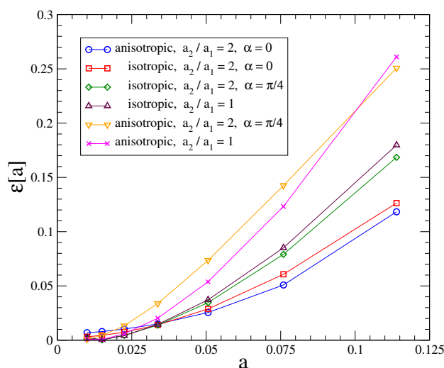
FIGURE 4. 2D Test case with nested inhomogeneities
