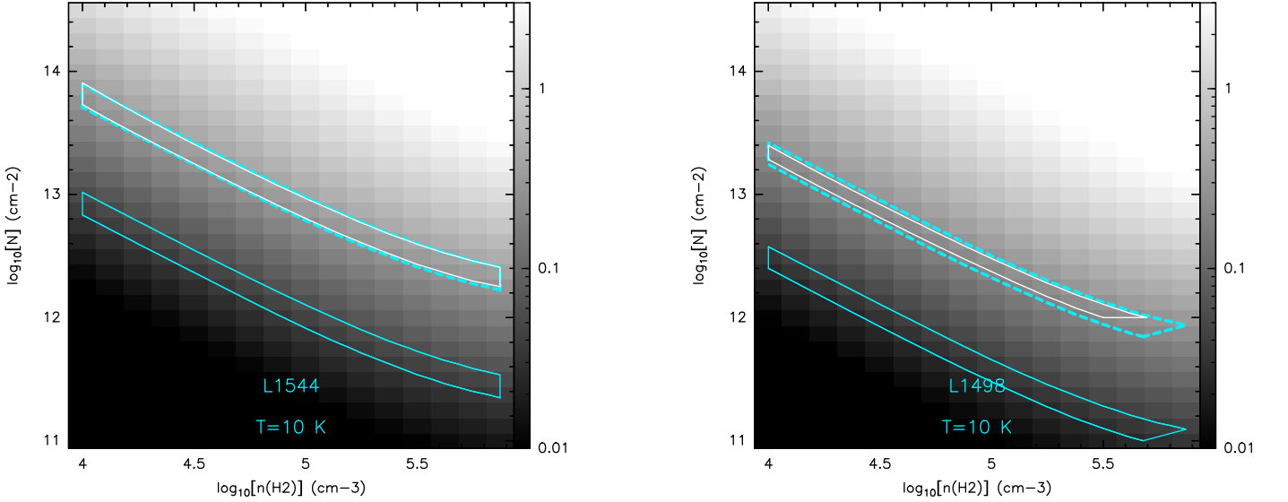
Fig. B.1. LVG predictions at T = 10 \text{ K} towards L1544 (left) and L1498 (right). In each panel, the grey scale shows the predicted intensity of the 110024.590 MHz component of the C 15 N(1-0) hyperfine multiplet. The boxes (full line) delineate the solutions for the C 15 N (cyan) and the 13 CN lines (white). The dashed box shows the C 15 N solutions when the C 15 N column density is multiplied by factors of 7.5 and 7 for L1544 and L1498 respectively.
