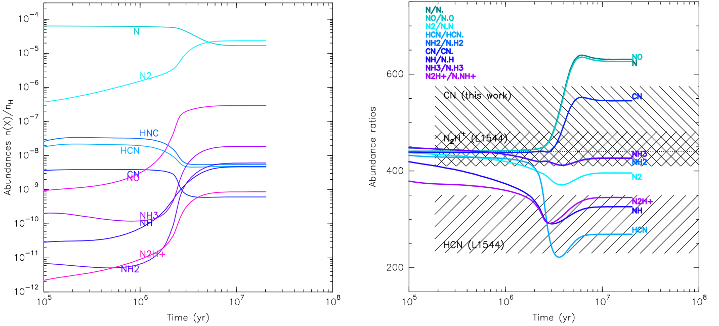
Fig. 1. Fractional abundances (left) and abundance ratios (right) of selected species. The observed isotopic ratios towards L1544 for HCN and CN, as well as towards L1498 for CN, are shown as hatched areas (right panel). The 15 N atom is noted N., such that CN. matches C 15 N, etc. The dotted line shows the adopted reference elemental isotopic ratio, 14 N/ 15 N=440 (Marty et al. 2011).
