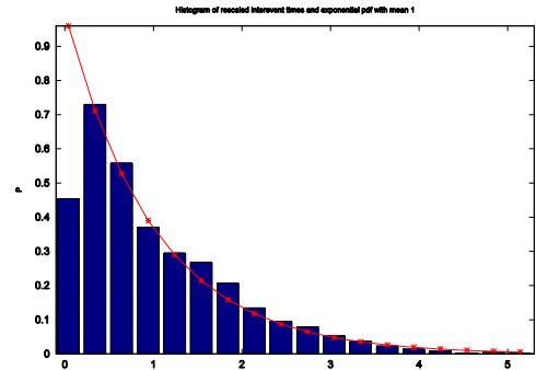
Figure 8: Histogram of the rescaled interevent times, and a pdf of an exponential distribution with mean=1
