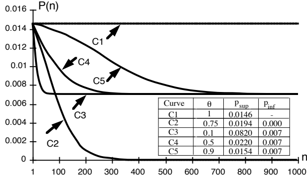
Figure 3: Probability of failure at execution for the discrete time hyperexponential model
