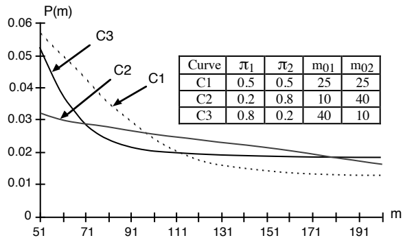
Figure 11: Estimation of P(m) in a specified execution profile
