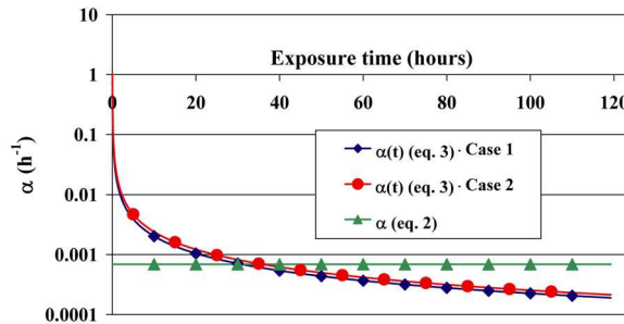
Figure 7: Evolution of the \alpha parameters in equations 2 and 3
