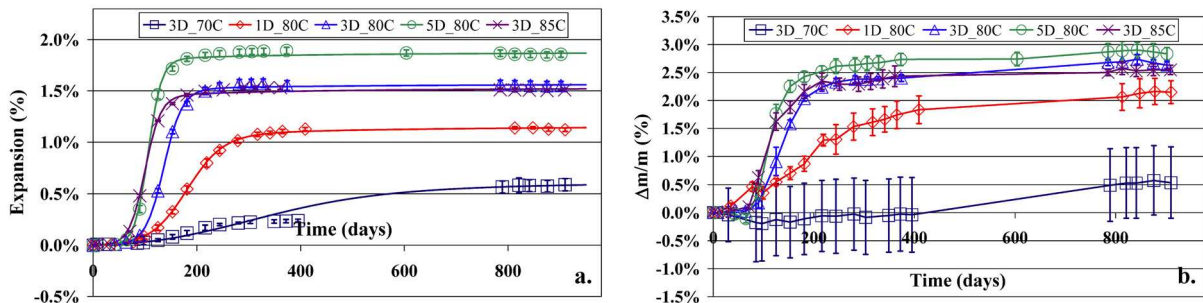
Figure 3: Expansion (a.) and mass monitoring (b.) of the specimens
