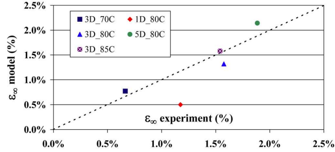
Figure 5: Comparison of the measured and predicted magnitudes of expansion according to equation 2
