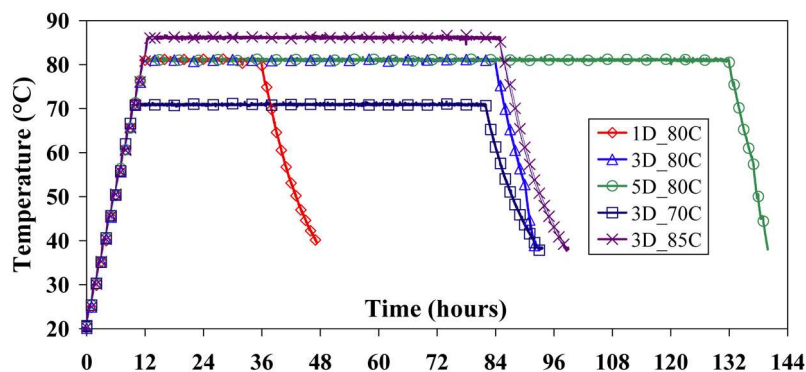
Figure 2: Temperature evolutions during the heat treatments
