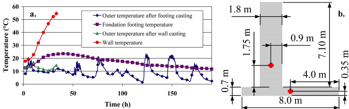
Figure 1 : Temperature monitoring (a) during the casting of an abutment (b) (location of the sensors marked by the crosses)
