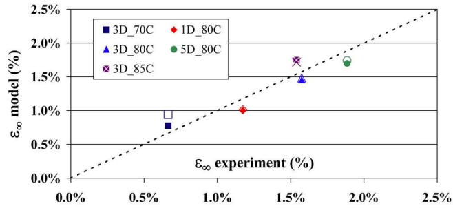
Figure 6: Comparison of the measured and predicted magnitudes of expansion according to equation 3 (hollow marks = case 1; plain marks = case 2)
