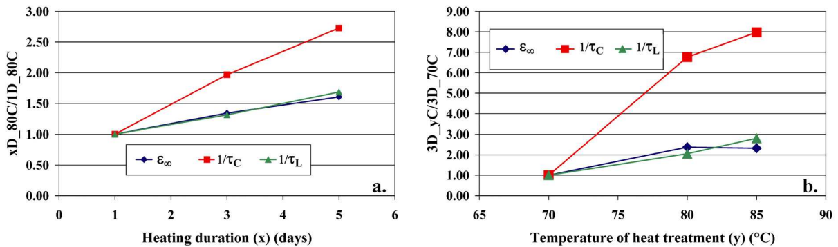
Figure 4: Effect of duration (a.) and temperature (b.) of the plateau of heat treatment on the magnitude and kinetics of expansion
