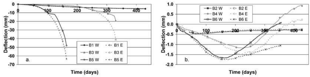
FIGURE 7: Mid span deflection of plain (a) and reinforced (b) beams (W = West; E = East).
