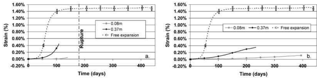
FIGURE 4: Vertical strain in the beams made of concrete AD at different depths (a. B5; b. B6).
