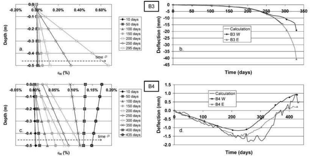
FIGURE 6: Mean longitudinal strain profiles (a and c) and comparison between the integration of their slopes and the deflection measured at mid span (b and d – W = West; E = East) for plain and reinforced beams affected by DEF (respectively B3 and B4).
