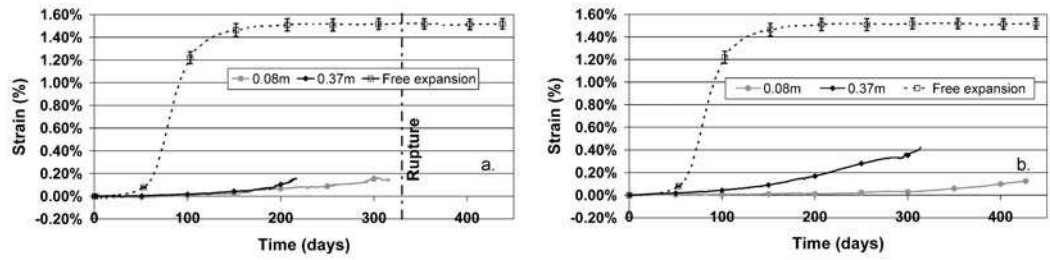
FIGURE 3: Vertical strain in the beams made of concrete D at different depths (a. B3; b. B4).
