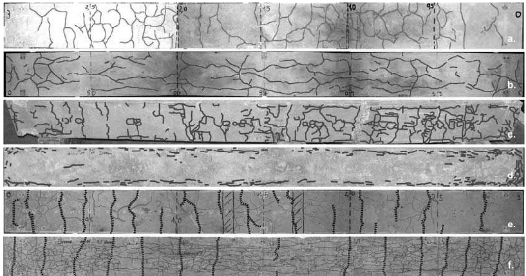
FIGURE 8: Cracking patterns of the beams at the end of the tests (a. lower face of B1, b. lower face of B2, c. lower face of B3, d. lower face of B4, e., upper face of B2, f. upper face of B4 – Map cracking on figures e and f corresponds to tests not described in this paper).
