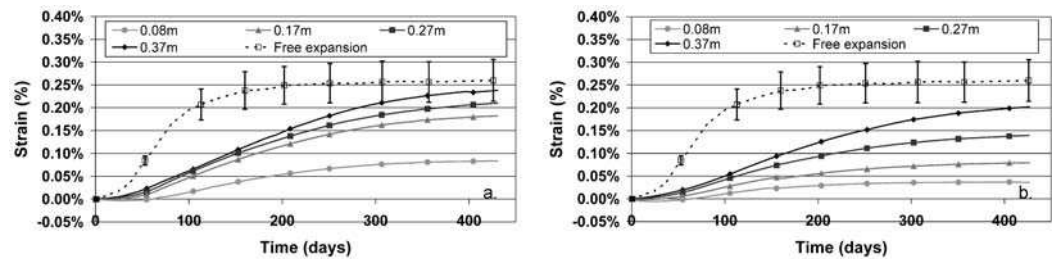
FIGURE 2: Vertical strain in the beams made of concrete A at different depths (a. B1; b. B2).
