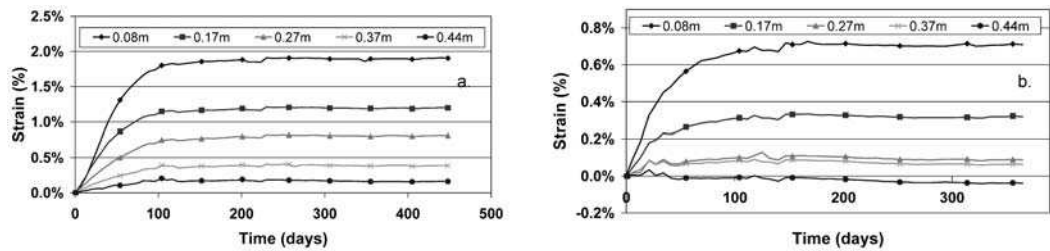
FIGURE 5: Residual expansion at various depths after failure of the beams B3 (a) and B5 (b).
