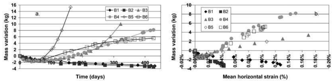
FIGURE 9: Global mass variation of the beams a. vs. time b. correlated to the mean longitudinal expansion.
