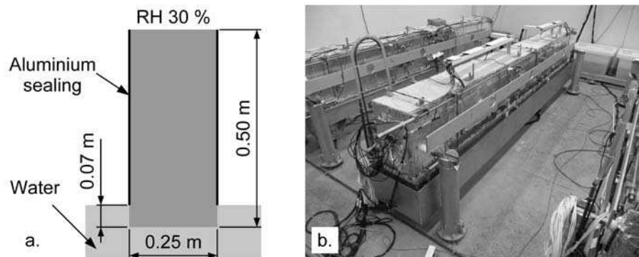
FIGURE 1: Water supply conditions during the test (a. cross section; b. general view).
