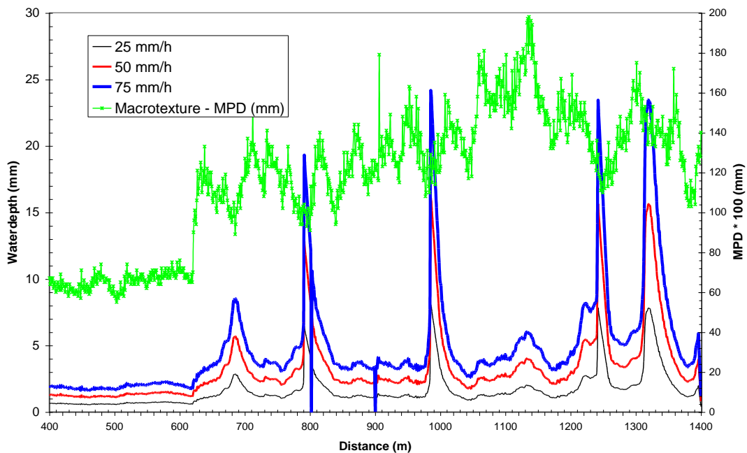
2 Figure 5 : Waterdepth for various rainfall intensity
