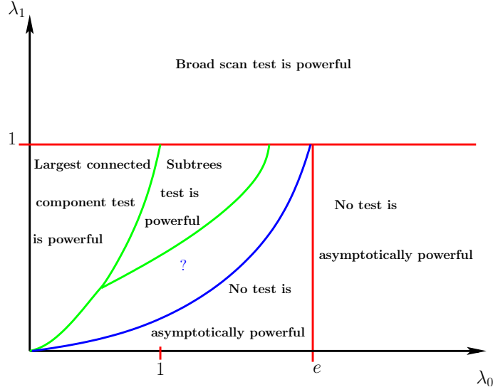
Figure 1: Detection diagram in the poissonian asymptotic where \lambda_0 and \lambda_1 are fixed and n = N^\kappa with 0 < \kappa < 1/2 .
