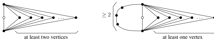
Fig. 2: Some graphs avoiding the bowtie. The white vertex is optional.
