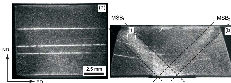
Fig. 1. MSB formation and shear deformation in copper samples deformed in channel-die. (a) initial position of scratches after 24% reduction. (b) bending of the scratches within MSB_1 and MSB_2 after further 25% deformation up to a final 50% reduction. Optical micrographs on longitudinal (ND-ED) plane
