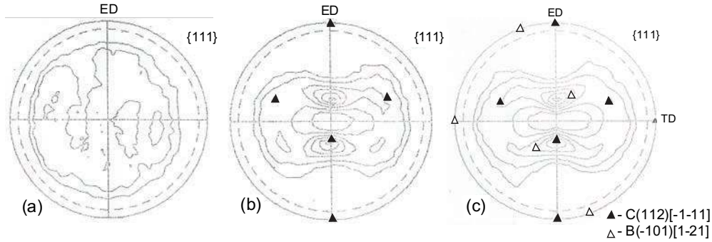
Fig. 2. X-ray diffraction \{111\} pole figures showing global texture development measured on the compression plane: (a) in initial material, (b) after 25% and (c) 50% compression in channel die
